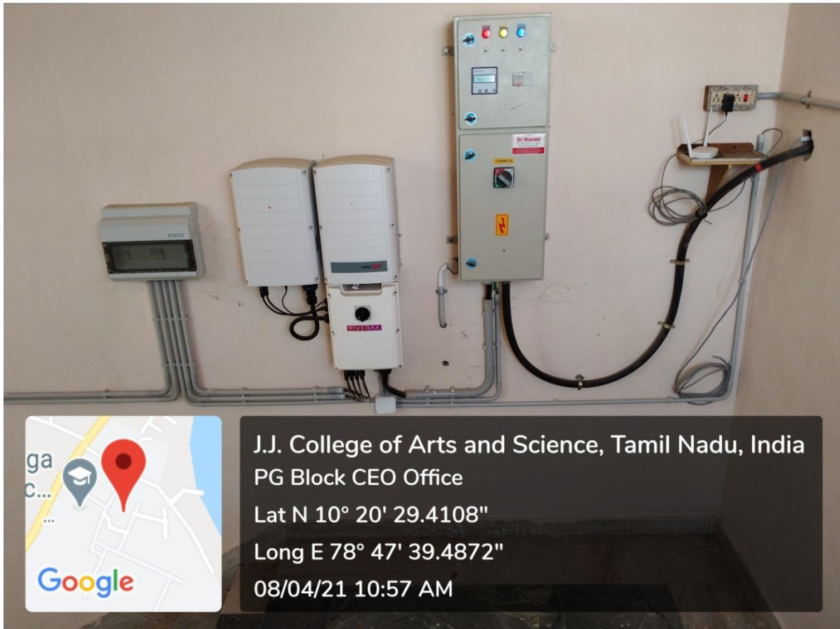
Wheeling to the Grid (Power converter from Solar energy)
